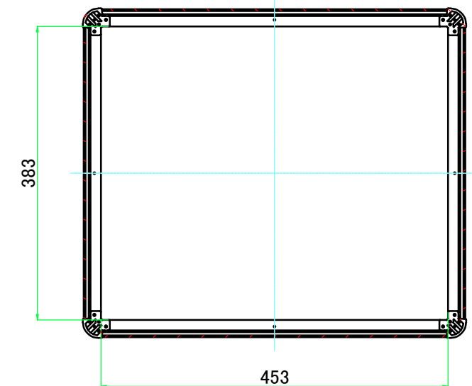
C-C (1:7)
